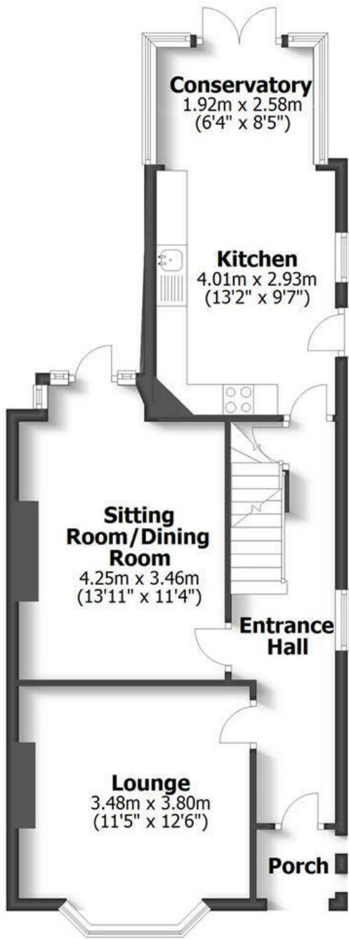
Ground Floor
